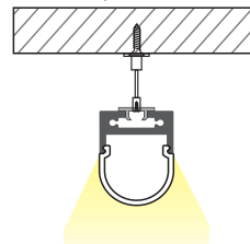
Installation method
