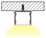
Installation method
